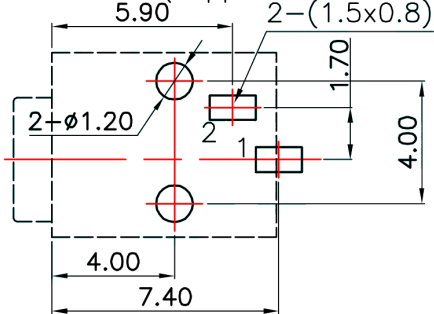
P.C.B LAYOUT(copper-sided view)
