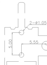
PCB LAND DIMENSION
