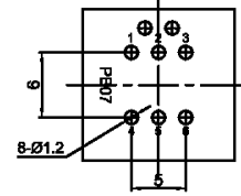
PCB HOLE(BOTTOM VIEW)
