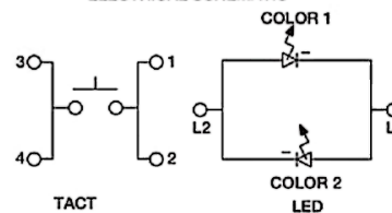
ELECTRICAL SCHEMATIC
