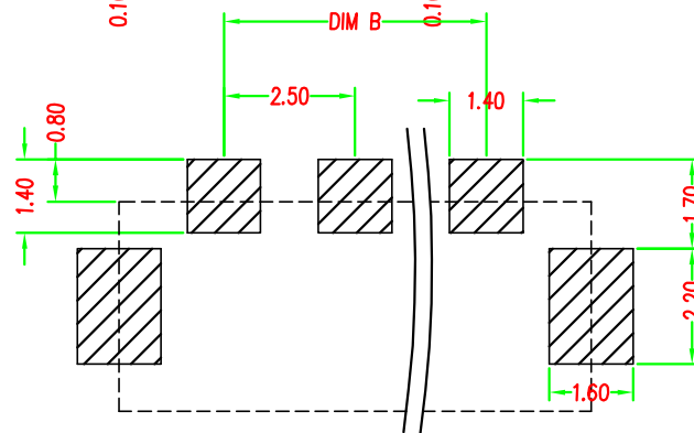
RECOMMENDED PCB LAYOUT TOL: (±0.05)
