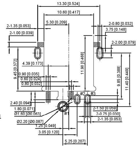
PCB LAYOUT TOP VIEW TOLERANCES: ±0.05
