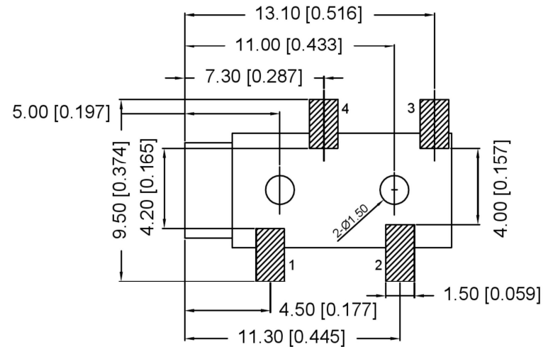
PCB LAYOUT TOP VIEW TOLERANCES :±0.05
