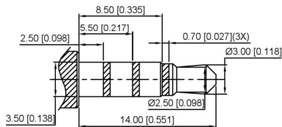
(Ø3.50mm 4 POLE PLUG DETAIL DRAWING)
