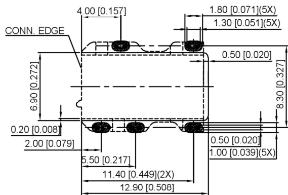
RECOMMENDED PCB LAYOUT (COMPONENT SIDE)
