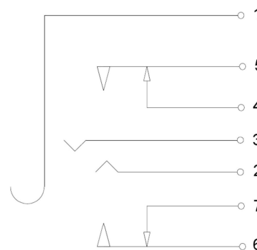
SCHEMATIC
