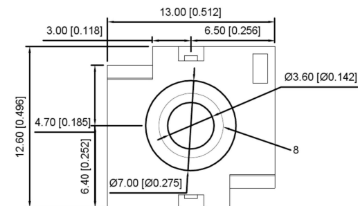
PJ-3440-2 Copper sleeve
