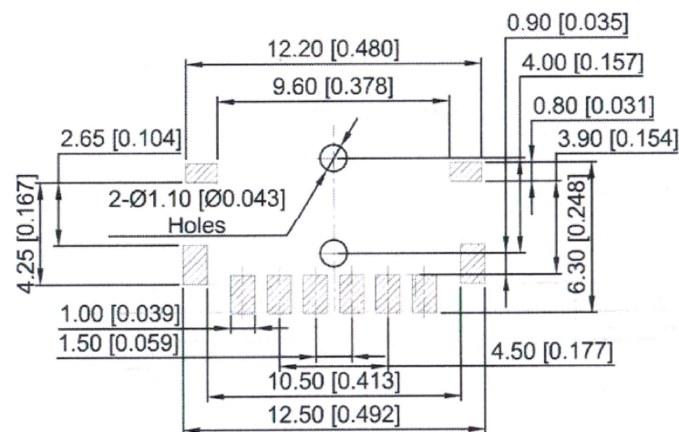
P.C.B Mounting Pattern Dimension
