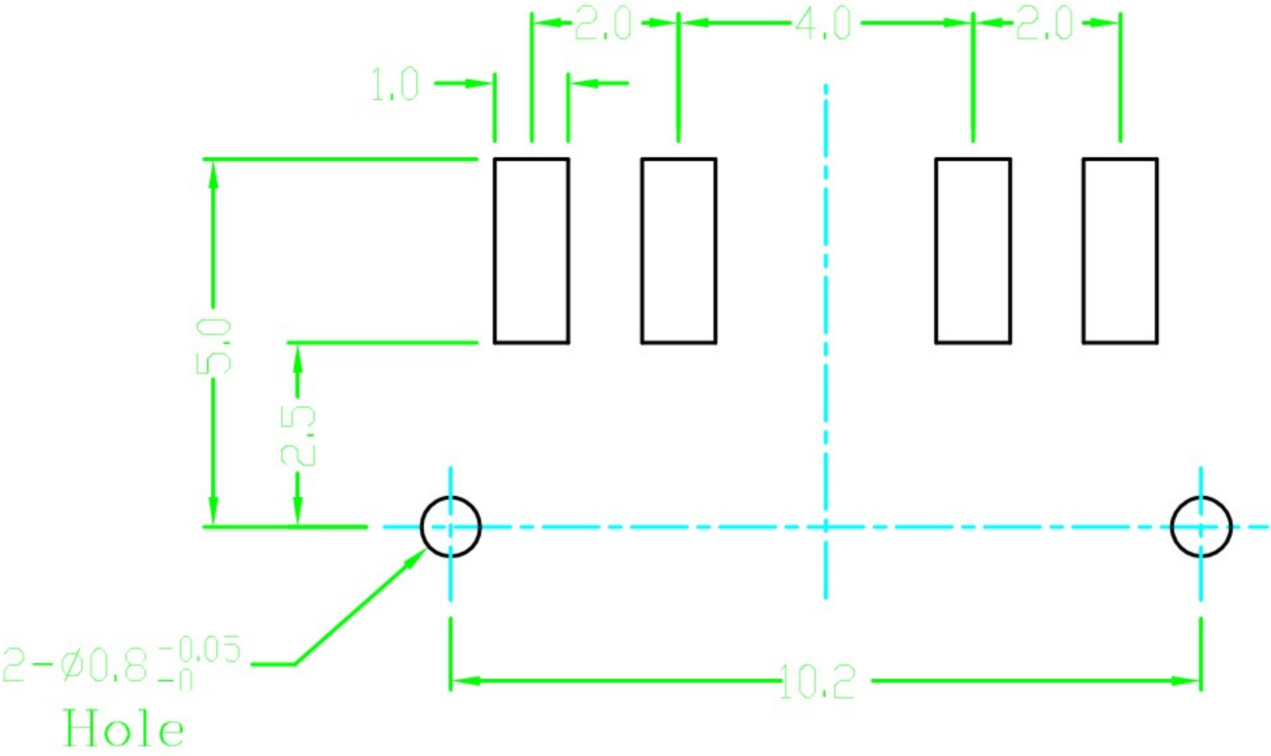
PCB LAYOUT VIEWED FROM DIRECTION A
