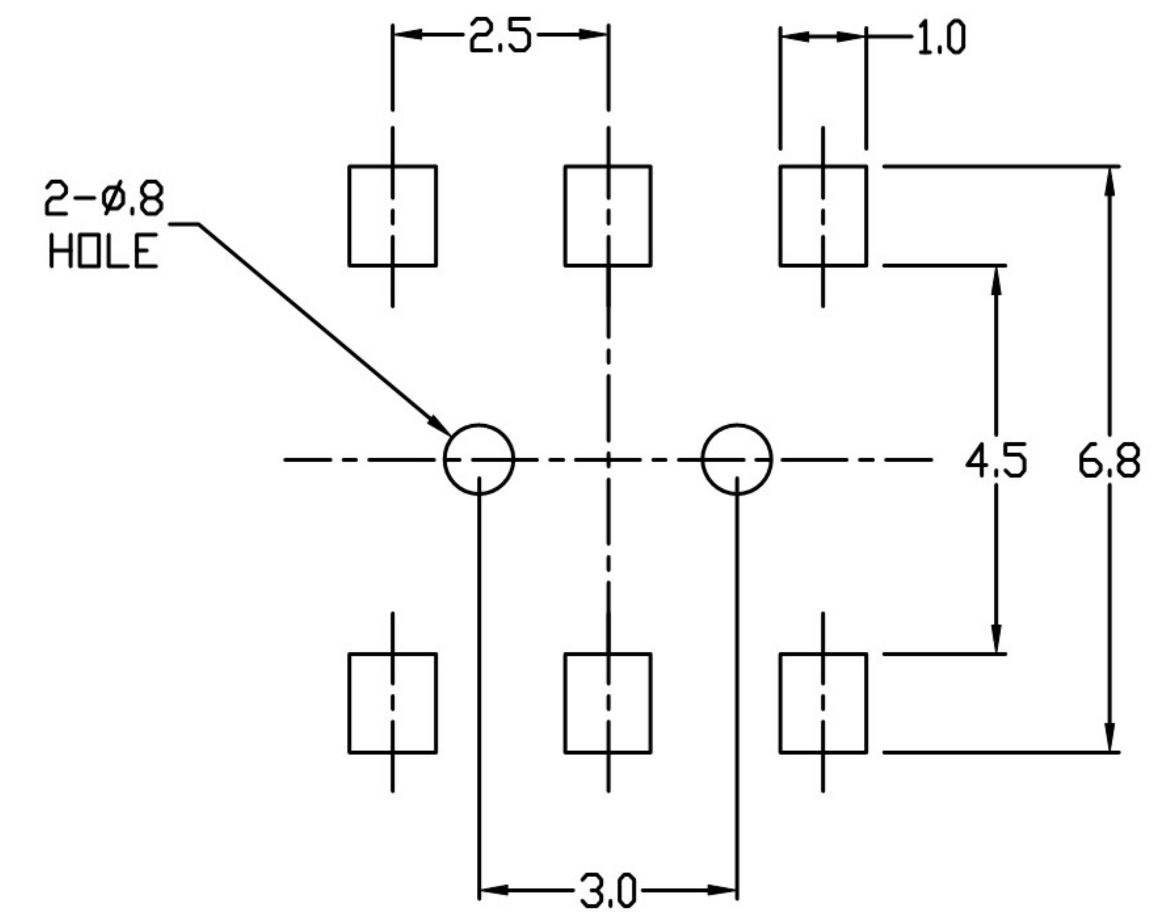
P.C. BOARD LAYOUT
