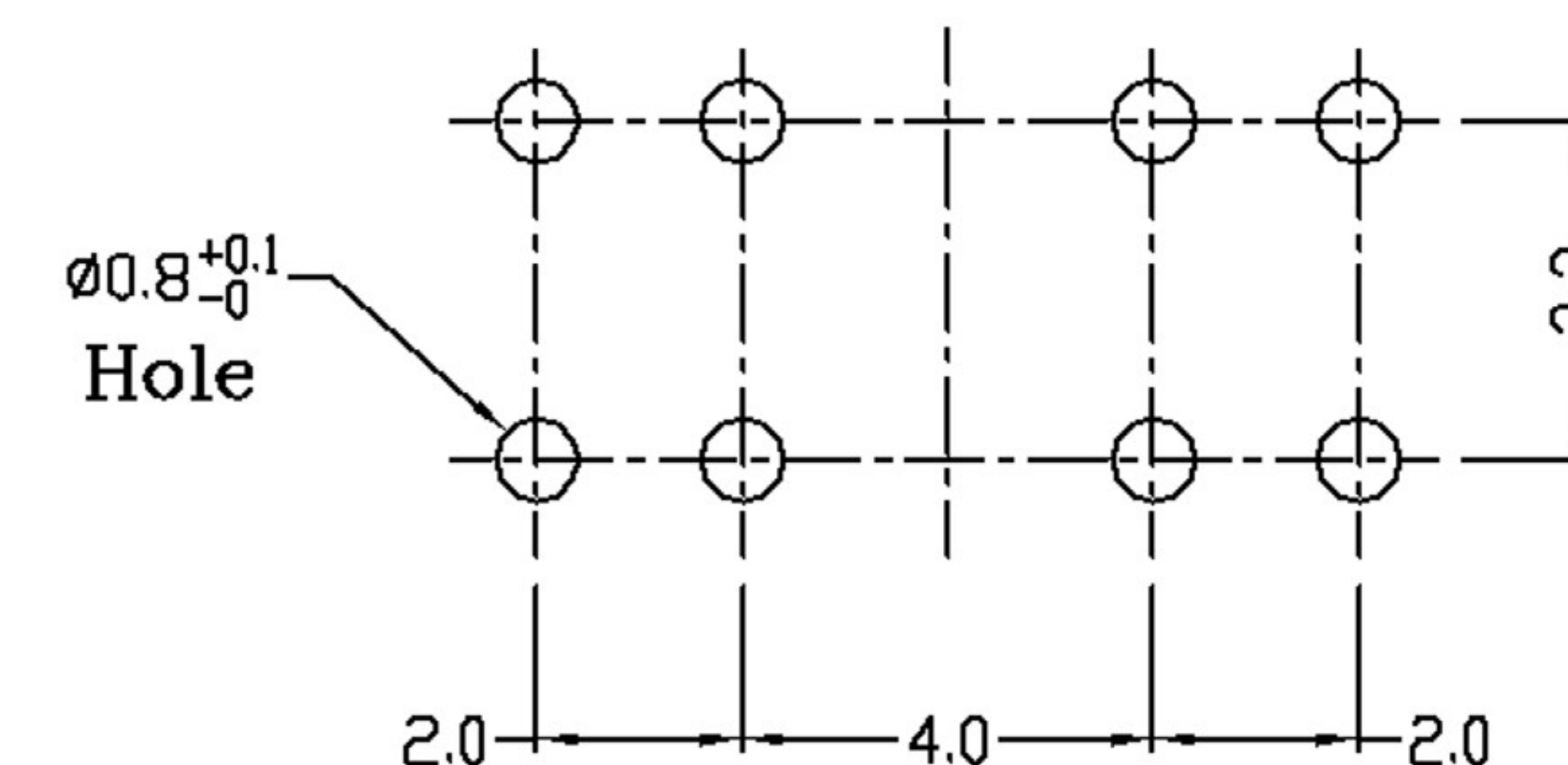
P.C. BOARD LAYOUT BOTTOM VIEW
