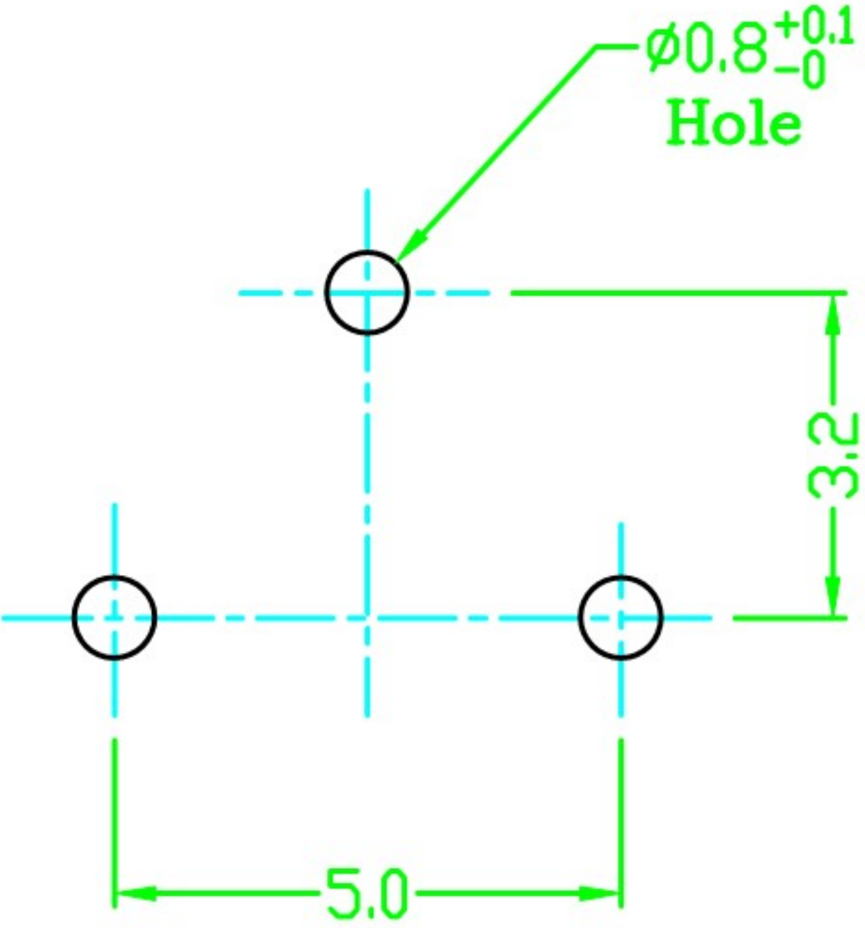
P.C. BOARD LAYOUT
