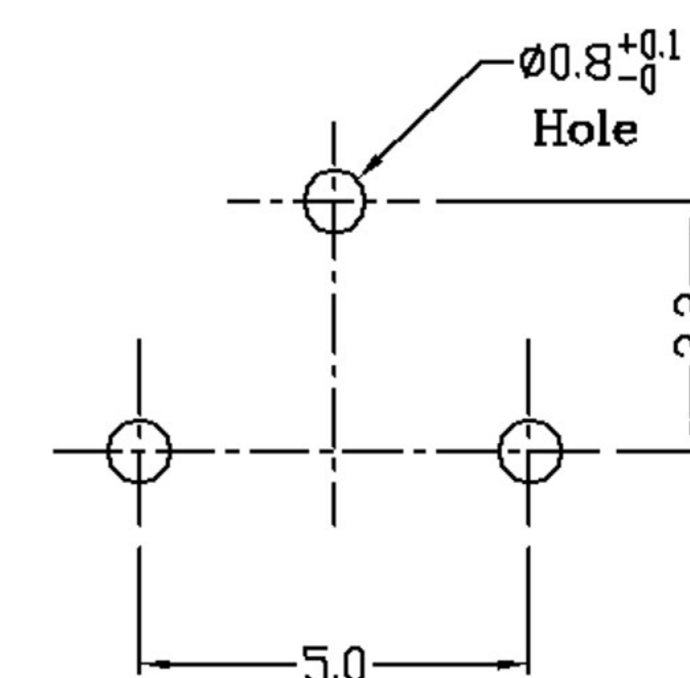
P.C. BOARD LAYOUT
