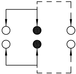
SCHEMATIC (NON-SHORTING)
