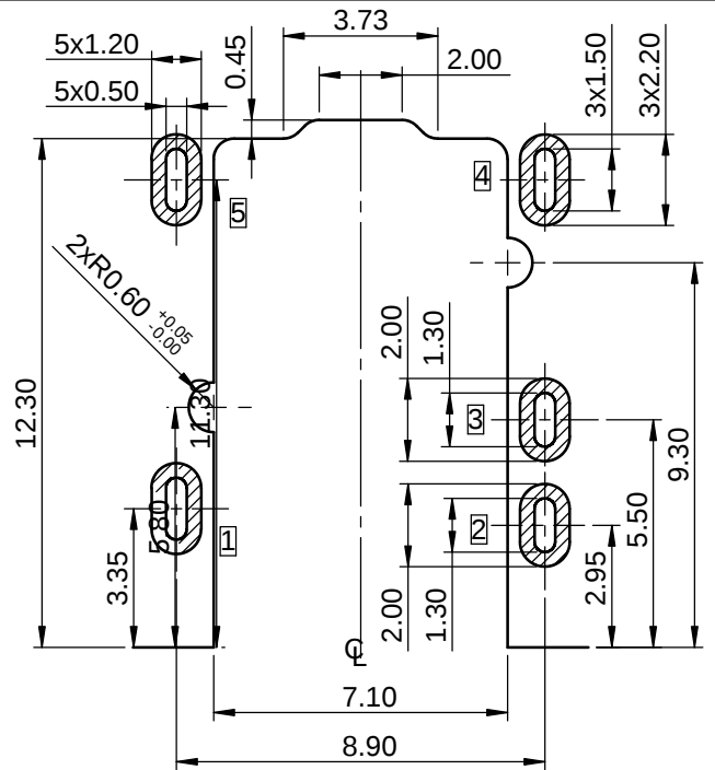
RECOMMENDED PCB LAYOUT(TOP VIEW) (GENERAL TOLERANCE \pm 0.05 )
