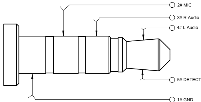
MALE PLUG SCHEMATIC
