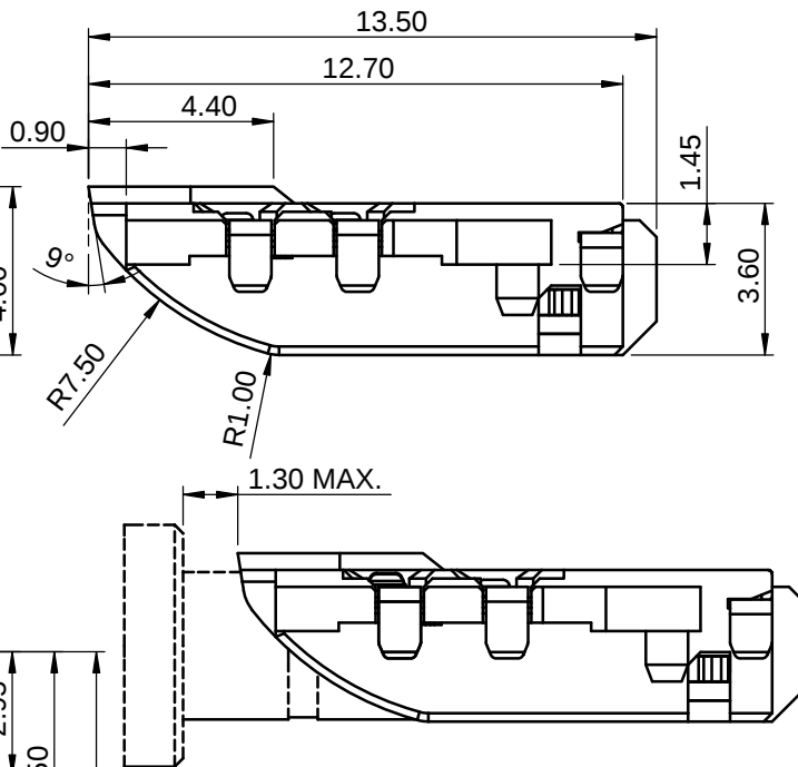
PLUG MATE DRAWING
