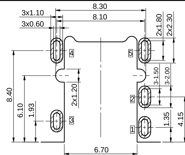
RECOMMENDED PCB LAYOUT(TOP VIEW) (GENERAL TOLERANCE \pm 0.05 )
