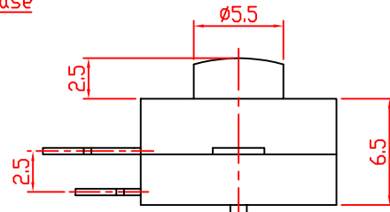
(E) Embossed Case
