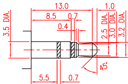
MATE PLUG
