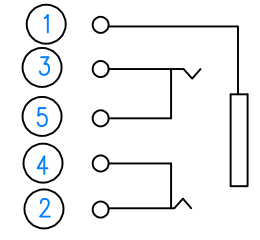
CIRCUIT
