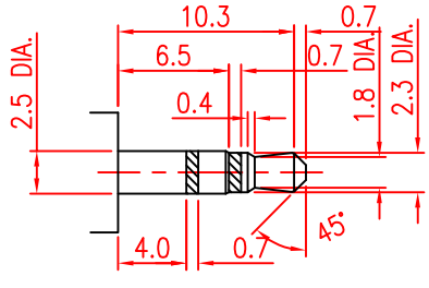
MATE PLUG
