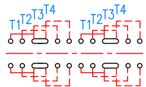
CIRCUIT
