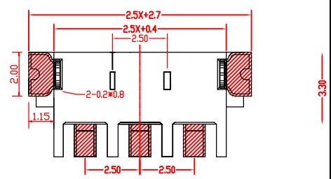
PCB LAYOUT (3pin)
