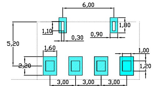
RECOMMENDED PCB LAYOUT TOP VIEW (.XX±0.05)
