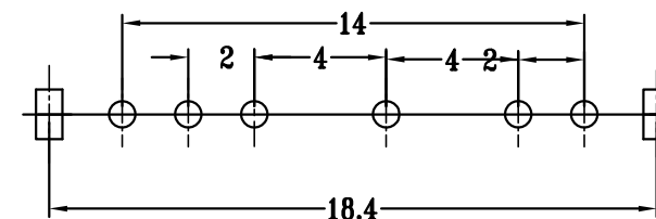
P.C.B LAYOUT BOTTOM VIEW
