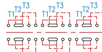
CIRCUIT
