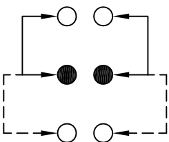
SCHEMATIC (NON-SHORTING)
