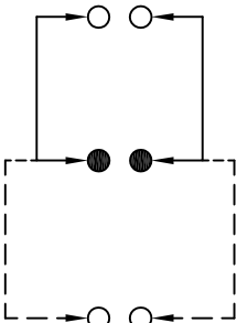
SCHEMATIC (NON-SHORTING)
