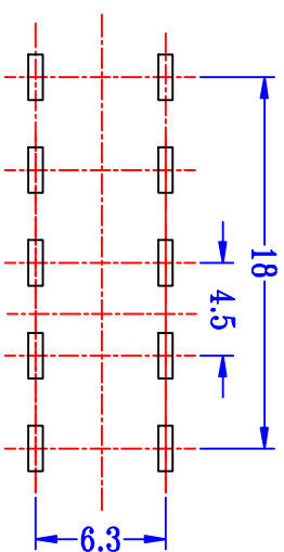
P.C.B LAYOUT BOTTOM VIEW
